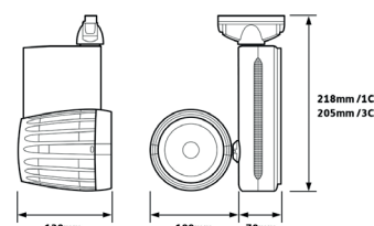
Side And Front Profile View Dimensions
