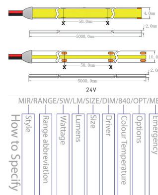
COB-FLEX Tape Dimensions
