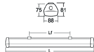
ECOLINE Dimensions
